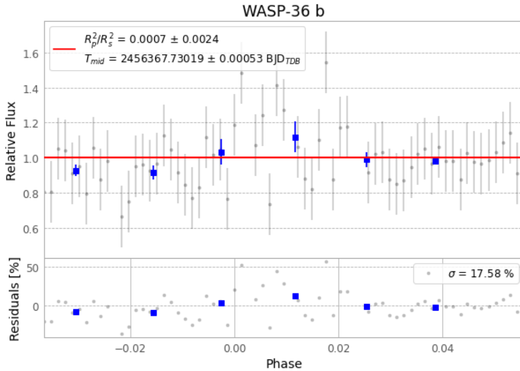
Figure 1 — FinalLightCurve_WASP-36 b_2013-03-15.png (SHA-256 f92723cd6fbd82a6...)
