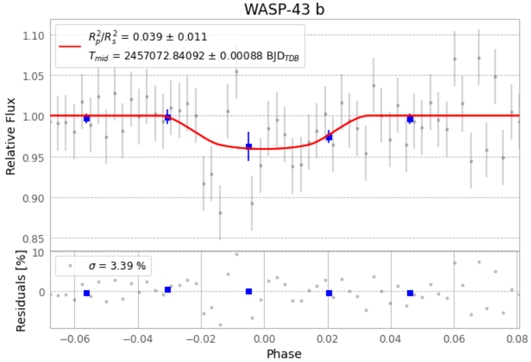
Figure 1 — FinalLightCurve_WASP-43 b_2015-02-18.png (SHA-256 420970f254564bae...)
