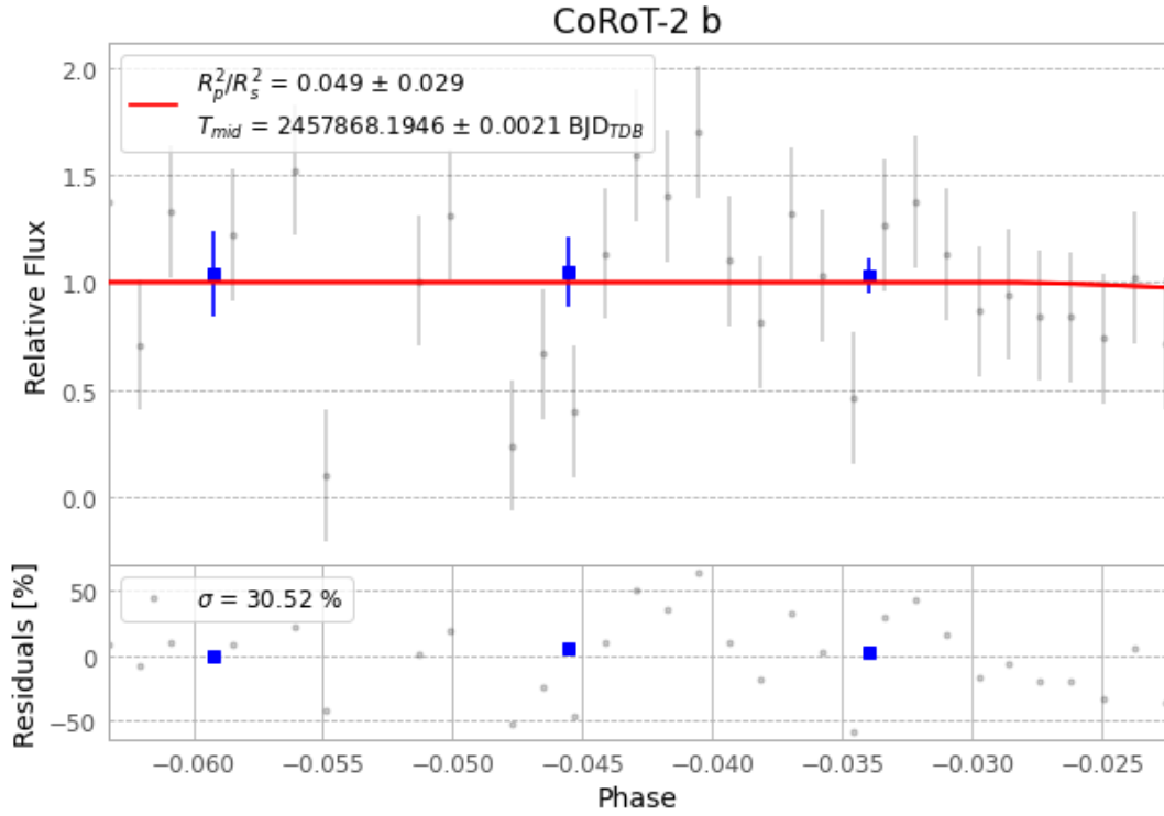
Figure 1 — FinalLightCurve_CoRoT-2 b_2017-04-26.png (SHA-256 cca78a043fbeb9bd...)
