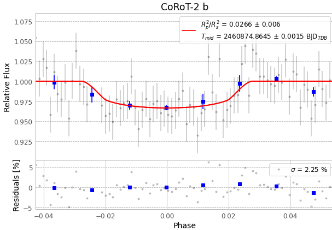
Figure 1 — FinalLightCurve_CoRoT-2 b_2025-07-17.png (SHA-256 71c07a5362efb6e6...)
