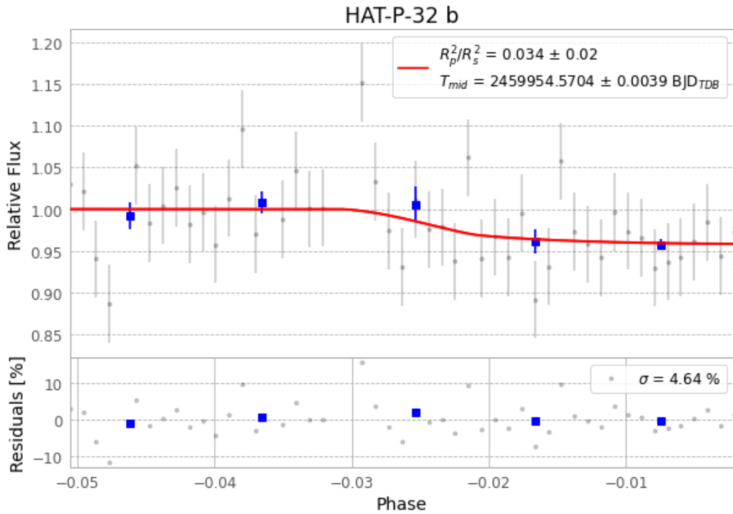
Figure 1 — FinalLightCurve_HAT-P-32 b_2023-01-11.png (SHA-256 c9f6bf0e43bc21d6...)
