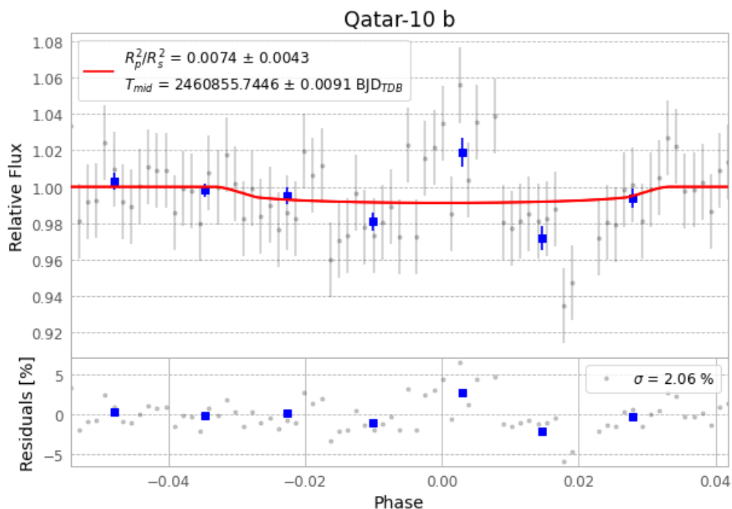
Figure 1 — FinalLightCurve_Qatar-10 b_2025-06-28.png (SHA-256 8830ad548d15624a...)
