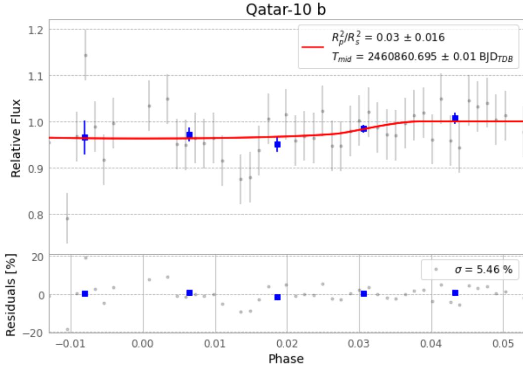
Figure 1 — FinalLightCurve_Qatar-10 b_2025-07-03.png (SHA-256 14bef2f349bc30e2...)
