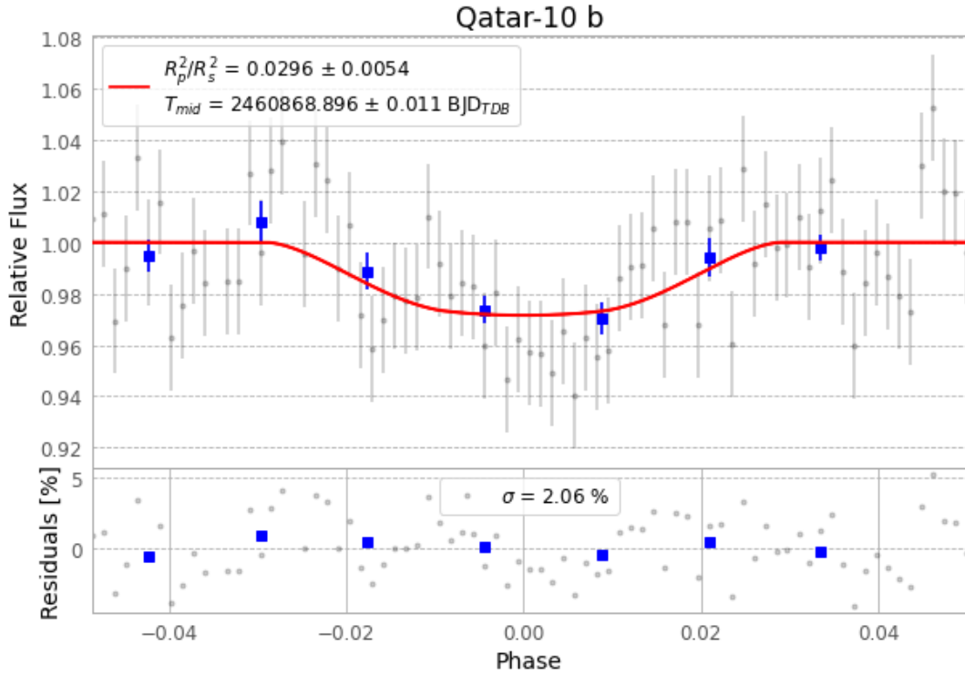
Figure 1 — FinalLightCurve_Qatar-10 b_2025-07-12.png (SHA-256 0b256f214893a48a...)
