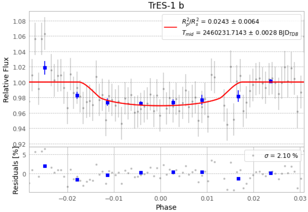
Figure 1 — FinalLightCurve_TrES-1 b_2023-10-13.png (SHA-256 9115679f746edb46...)
