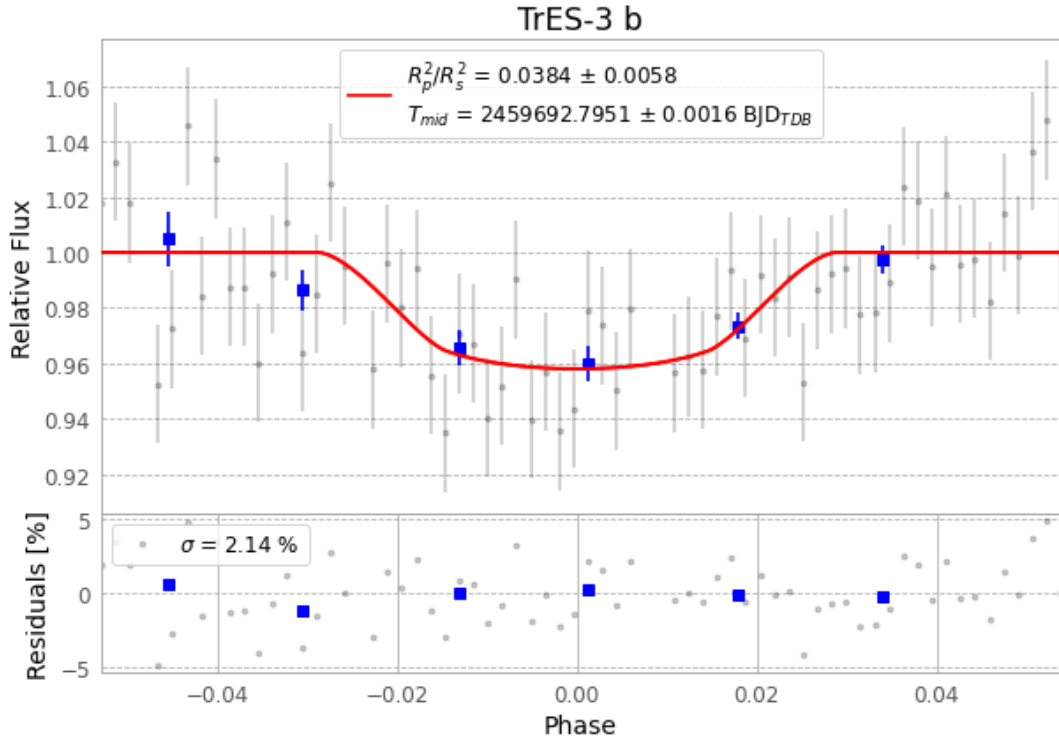
Figure 1 — FinalLightCurve_TrES-3 b_2022-04-22.png (SHA-256 8f06d46e2b036865...)
