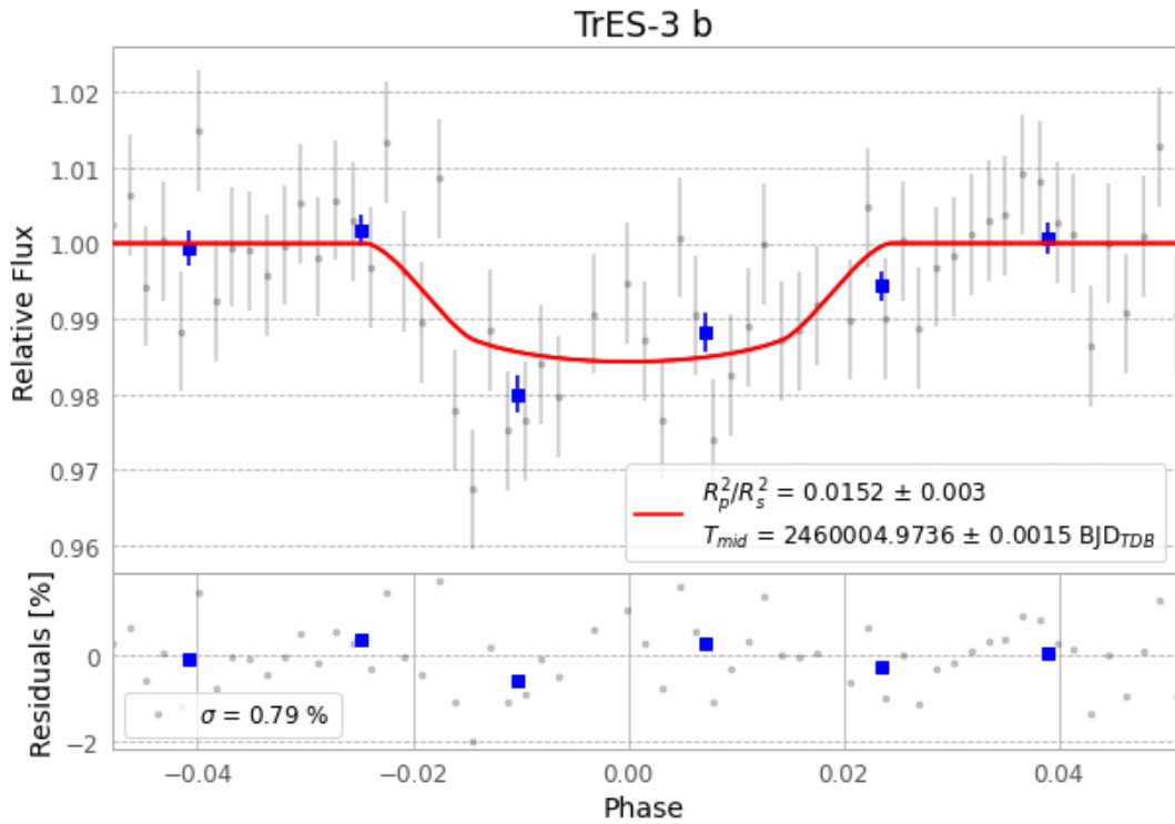
Figure 1 — FinalLightCurve_TrES-3 b_2023-03-01.png (SHA-256 a15fddfed9d5a1fe...)
