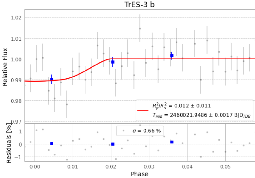
Figure 1 — FinalLightCurve_TrES-3 b_2023-03-18.png (SHA-256 17e1f7934d2a9355...)
