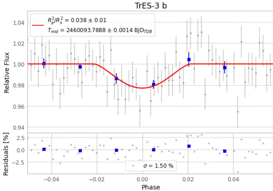
Figure 1 — FinalLightCurve_TrES-3 b_2023-05-28.png (SHA-256 c9f2b3fd5fcfad2b...)
