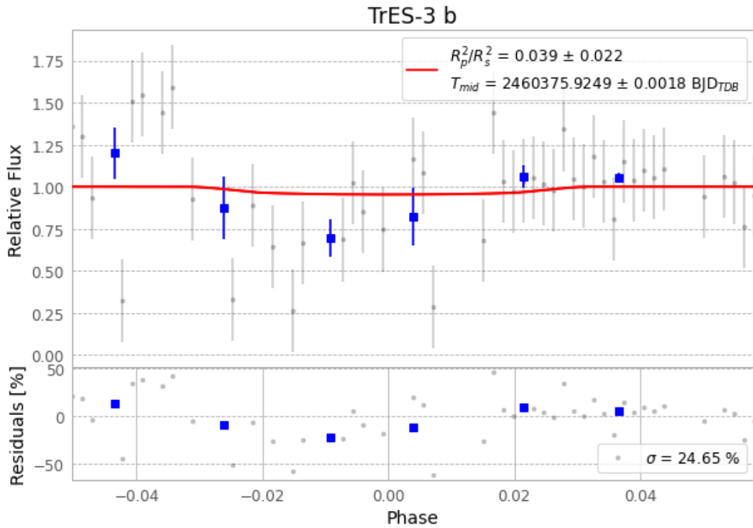
Figure 1 — FinalLightCurve_TrES-3 b_2024-03-06.png (SHA-256 c81a265a4e374d72...)
