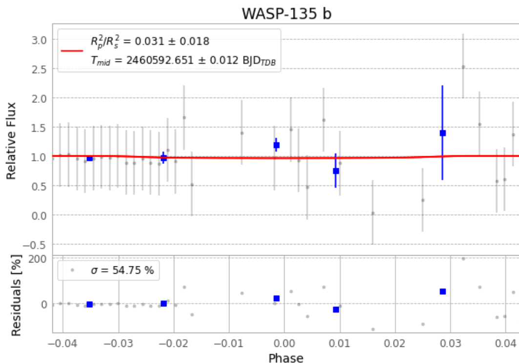
Figure 1 — FinalLightCurve_WASP-135 b_2024-10-08.png (SHA-256 0d3d31c84dc90921...)
