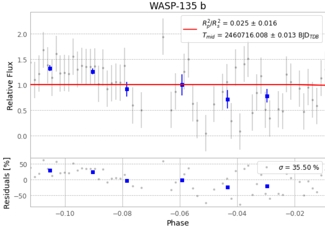
Figure 1 — FinalLightCurve_WASP-135 b_2025-02-09.png (SHA-256 2987f63394e5386c...)
