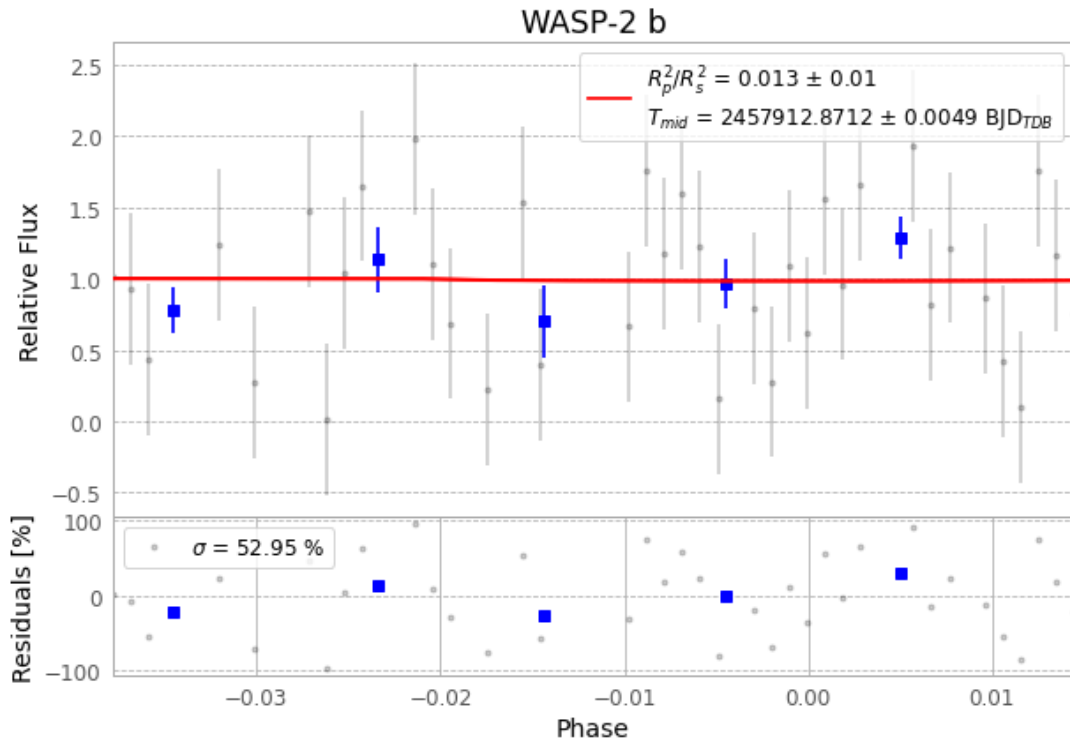
Figure 1 — FinalLightCurve_WASP-2 b_2017-06-07.png (SHA-256 3952e3d651e91d75...)
