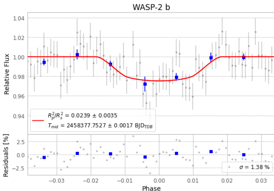
Figure 1 — FinalLightCurve_WASP-2 b_2018-09-15.png (SHA-256 7c3a1284c48e5ec6...)
