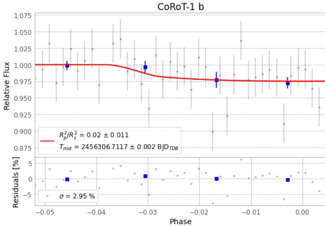
Figure 1 — FinalLightCurve_CoRoT-1 b_2013-01-13.png (SHA-256 29d07bf94844902e...)
