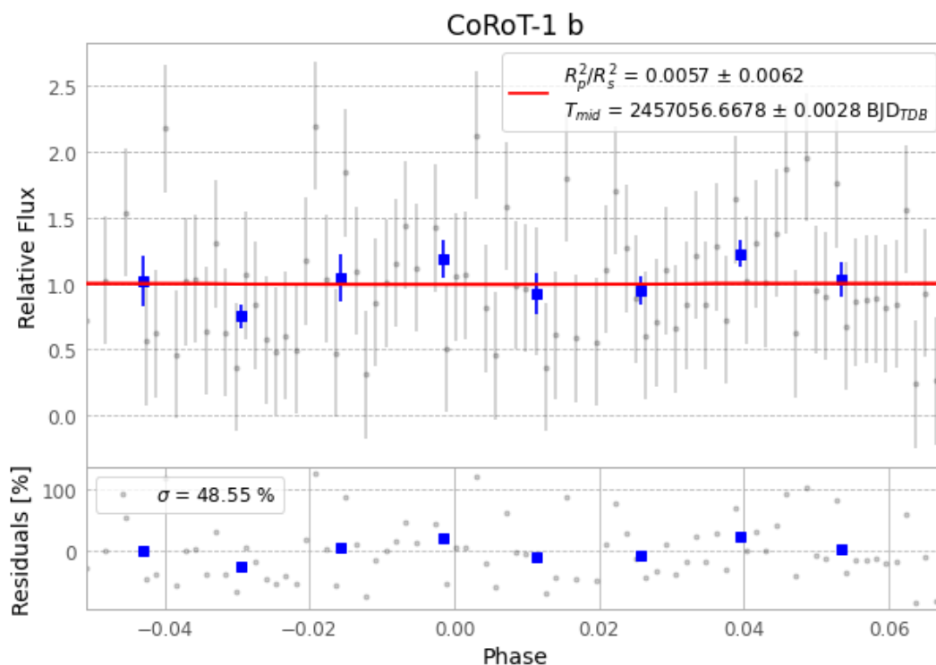
Figure 1 — FinalLightCurve_CoRoT-1 b_2015-02-02.png (SHA-256 ba4ccb6d3e19b27e...)
