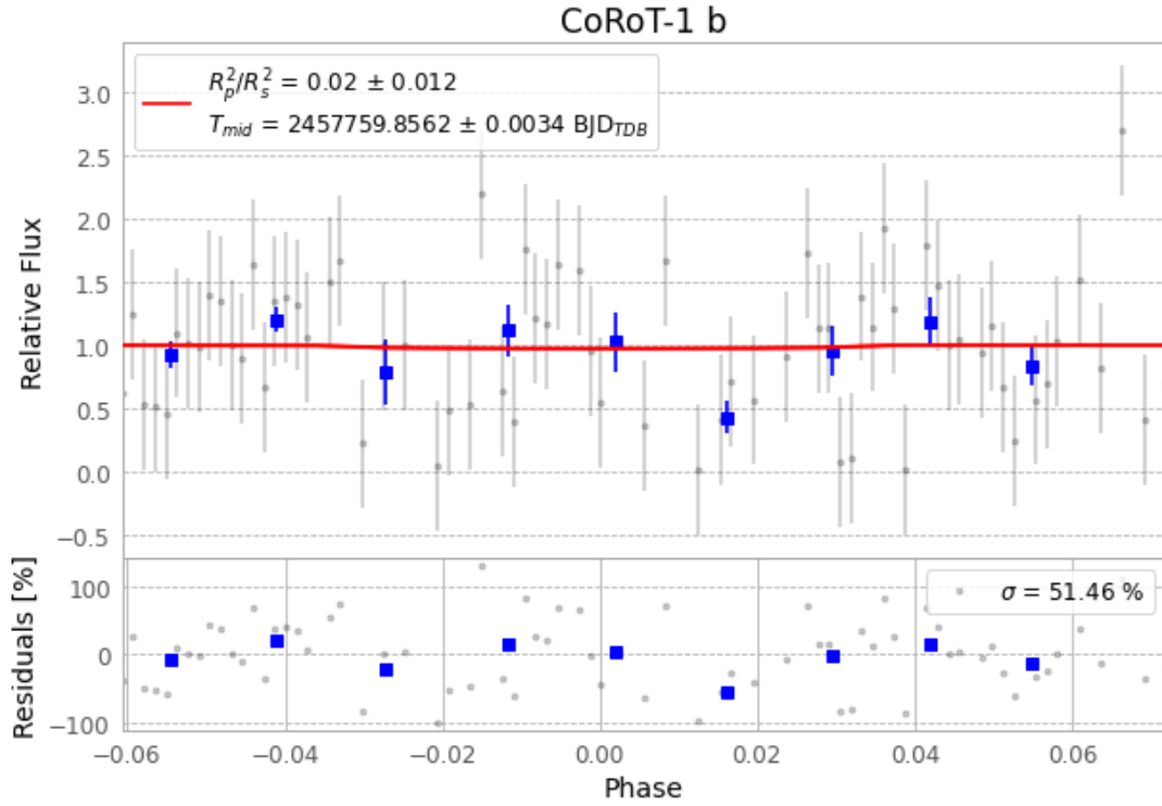
Figure 1 — FinalLightCurve_CoRoT-1 b_2017-01-05.png (SHA-256 8db5127231ea9190...)
