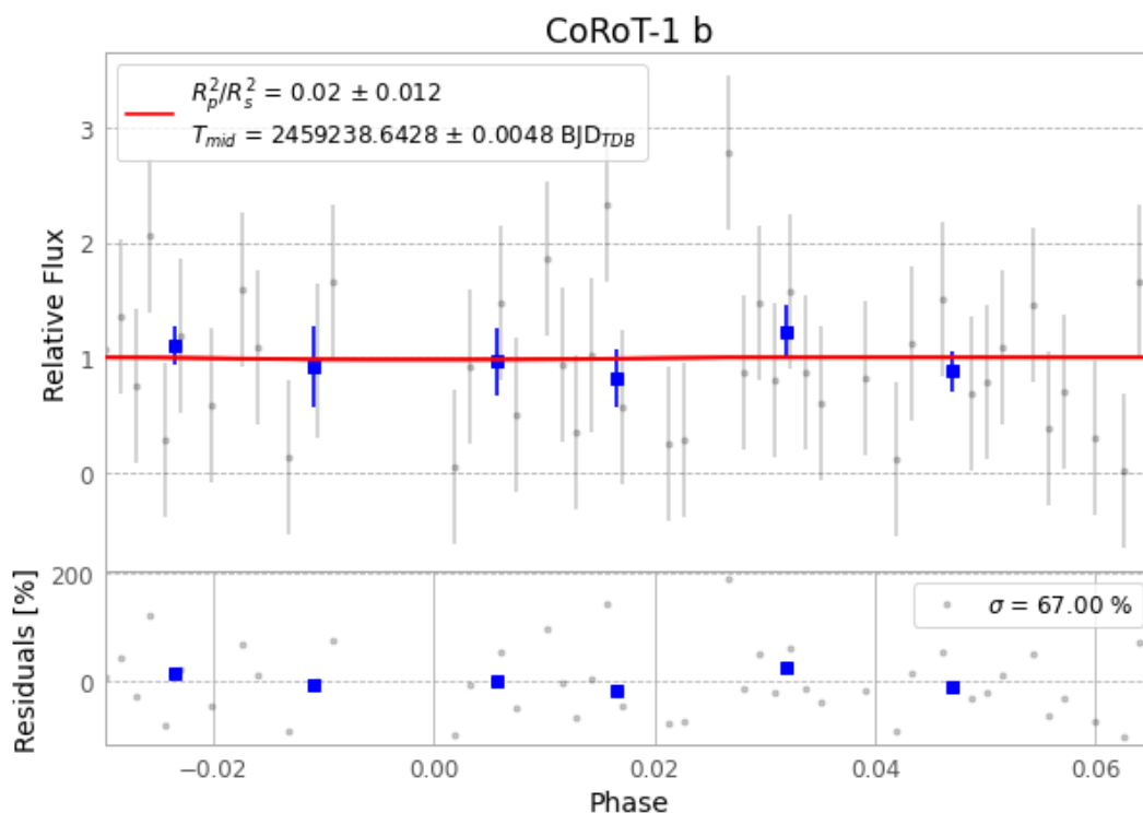
Figure 1 — FinalLightCurve_CoRoT-1 b_2021-01-23.png (SHA-256 b00ba35b6b8fb6e4...)
