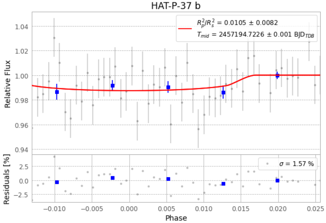
Figure 1 — FinalLightCurve_HAT-P-37 b_2015-06-20.png (SHA-256 de032007cf96ce56...)
