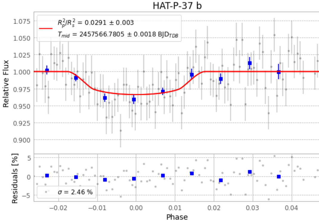
Figure 1 — FinalLightCurve_HAT-P-37 b_2016-06-26.png (SHA-256 e0630fa5f81d12a7...)
