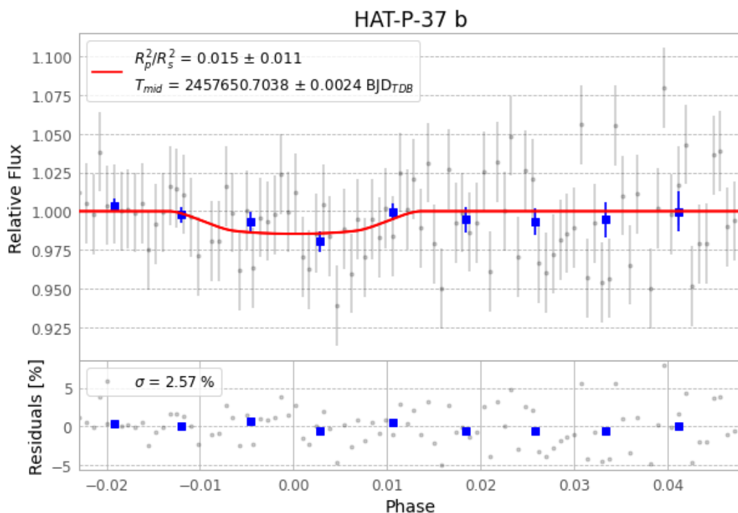
Figure 1 — FinalLightCurve_HAT-P-37 b_2016-09-18.png (SHA-256 f4d8113c37c69c08...)
