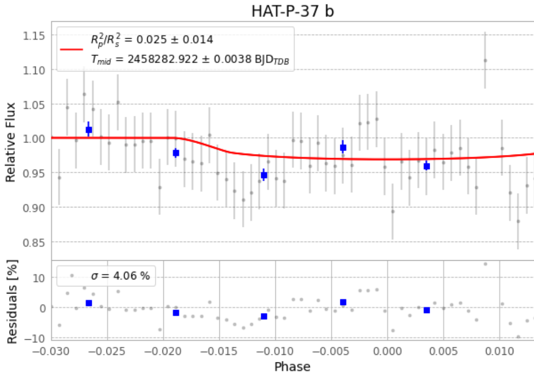
Figure 1 — FinalLightCurve_HAT-P-37 b_2018-06-13.png (SHA-256 39a5532beda61144...)
