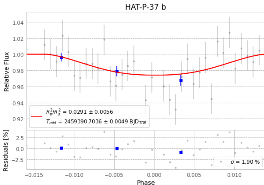
Figure 1 — FinalLightCurve_HAT-P-37 b_2021-06-24.png (SHA-256 f925e1d02fd57000...)
