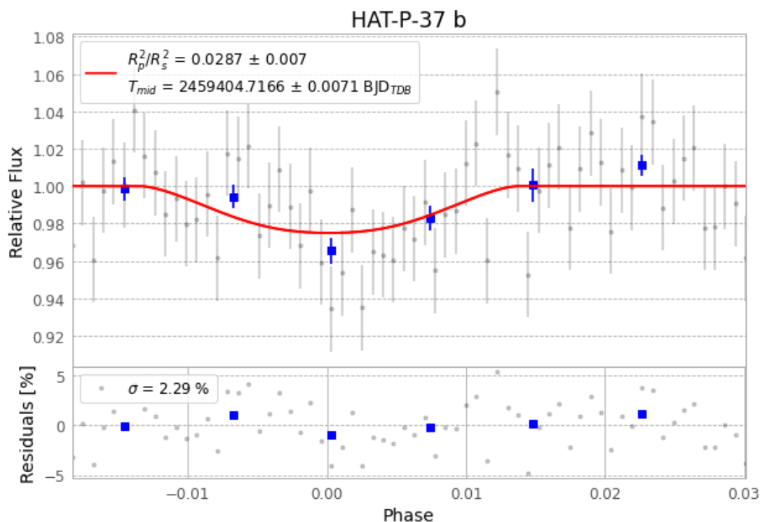
Figure 1 — FinalLightCurve_HAT-P-37 b_2021-07-08.png (SHA-256 d6d734c496aded5b...)
