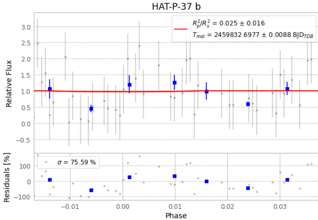
Figure 1 — FinalLightCurve_HAT-P-37 b_2022-09-09.png (SHA-256 68654a3ce5ea0956...)
