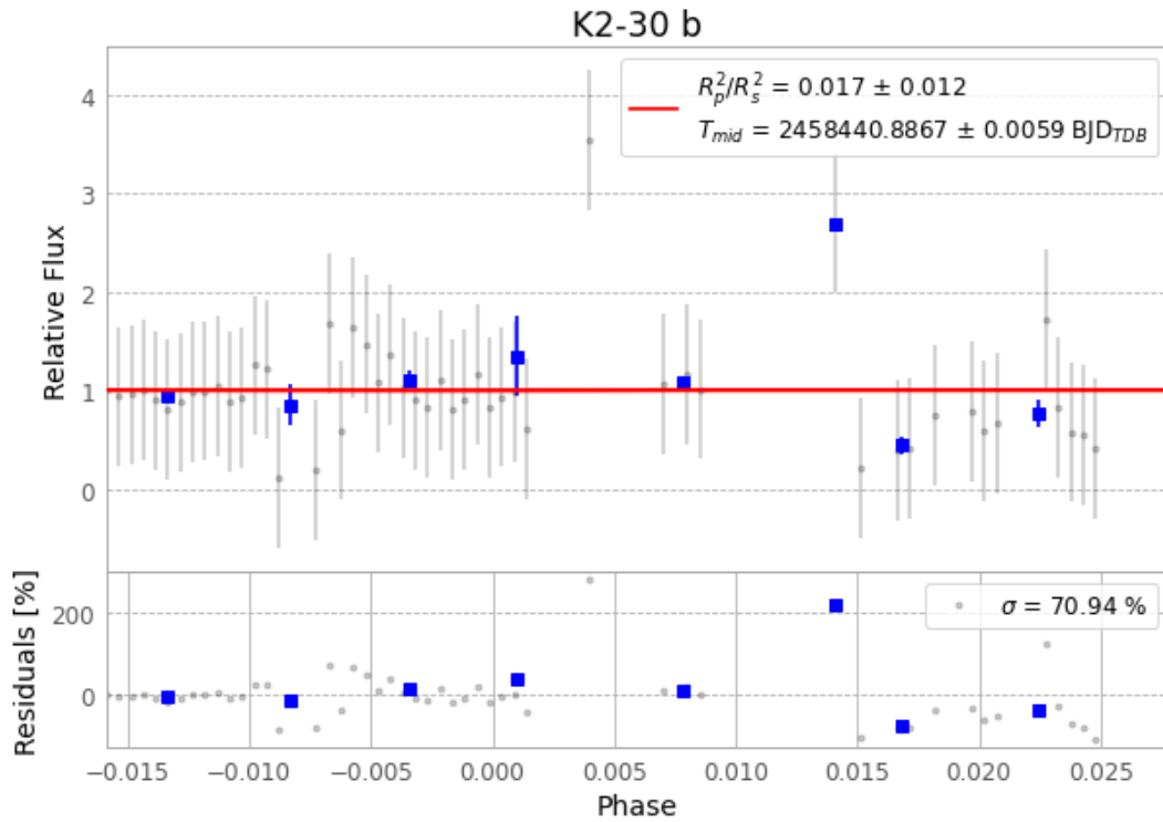
Figure 1 — FinalLightCurve_K2-30 b_2018-11-18.png (SHA-256 175cb44a89fbabd9...)
