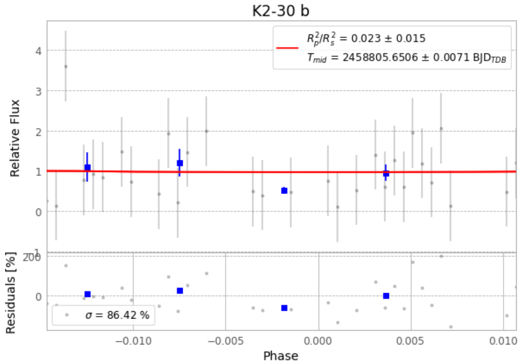
Figure 1 — FinalLightCurve_K2-30 b_2019-11-17.png (SHA-256 39aa3623e478b59a...)
