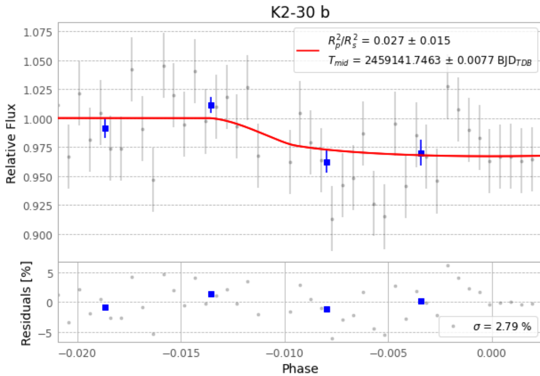
Figure 1 — FinalLightCurve_K2-30 b_2020-10-18.png (SHA-256 fe89cfb87604f113...)
