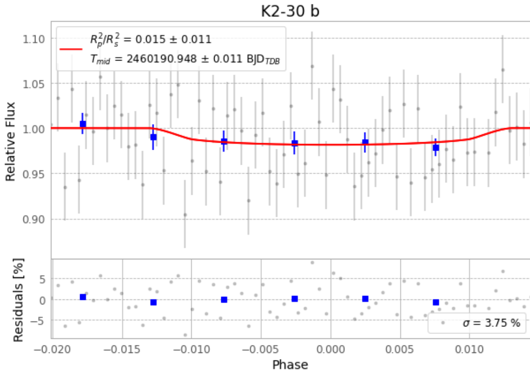
Figure 1 — FinalLightCurve_K2-30 b_2023-09-03.png (SHA-256 7f51d12ef4bbfca2...)
