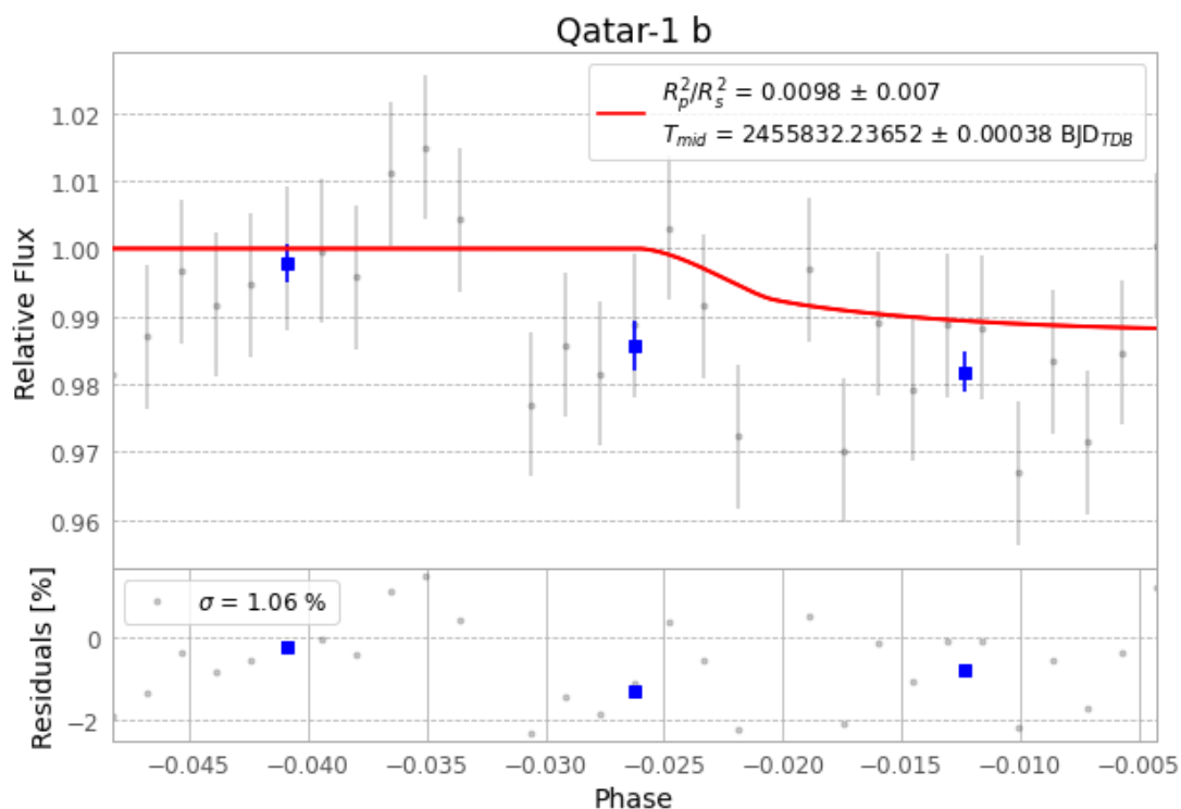
Figure 1 — FinalLightCurve_Qatar-1 b_2011-09-28.png (SHA-256 5a8c424d4ba0894a...)
