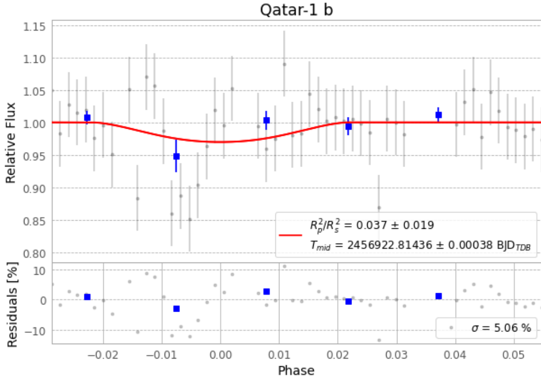
Figure 1 — FinalLightCurve_Qatar-1 b_2014-09-21.png (SHA-256 b7ca0bc7d13d4ec3...)
