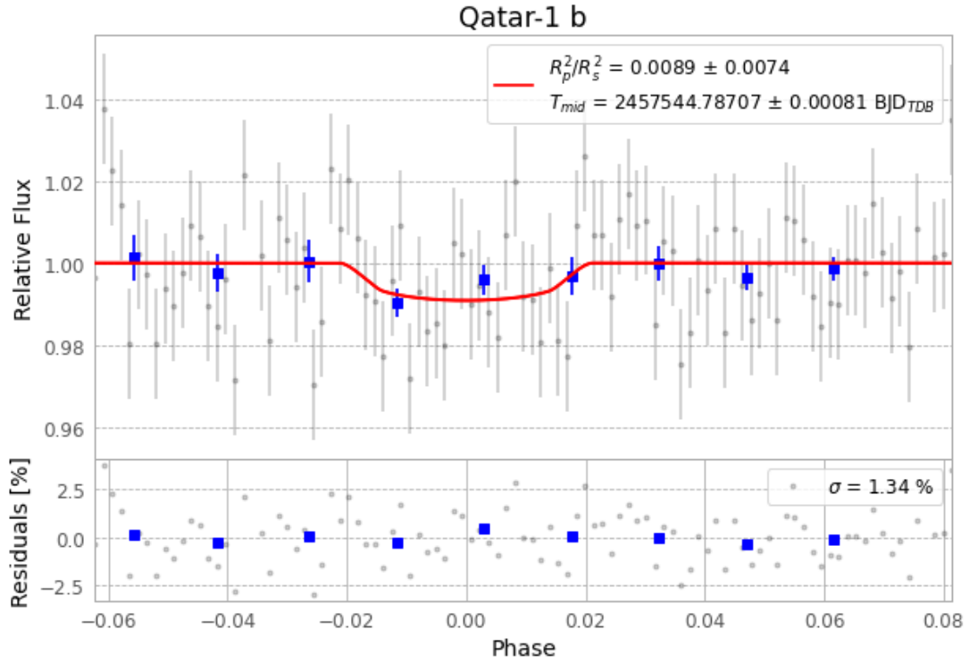
Figure 1 — FinalLightCurve_Qatar-1 b_2016-06-04.png (SHA-256 dcf68d4e41660e3b...)
