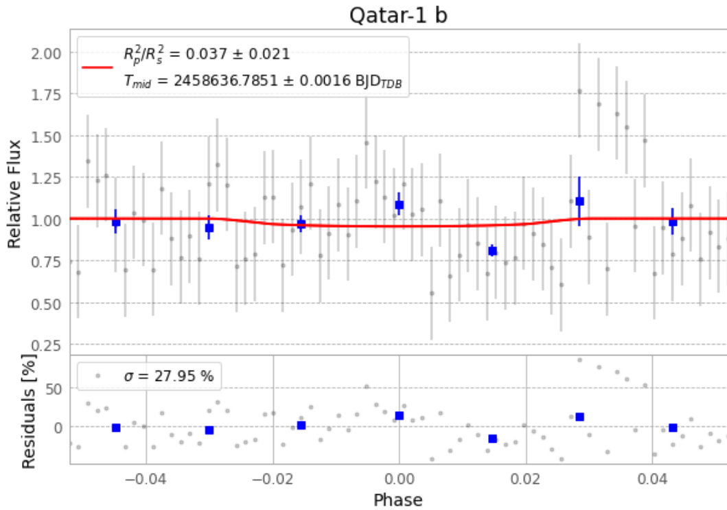
Figure 1 — FinalLightCurve_Qatar-1 b_2019-06-01.png (SHA-256 c37014c21b5b5bd5...)
