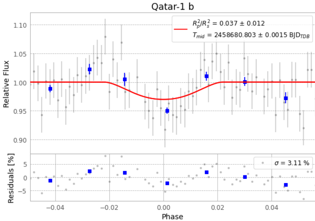
Figure 1 — FinalLightCurve_Qatar-1 b_2019-07-15.png (SHA-256 f71e2c1d5de1b81d...)
