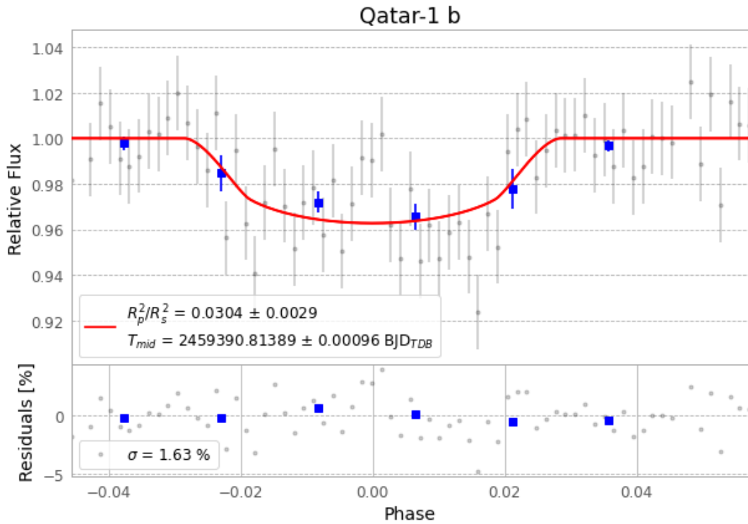
Figure 1 — FinalLightCurve_Qatar-1 b_2021-06-24.png (SHA-256 f5f07178e9556ee8...)
