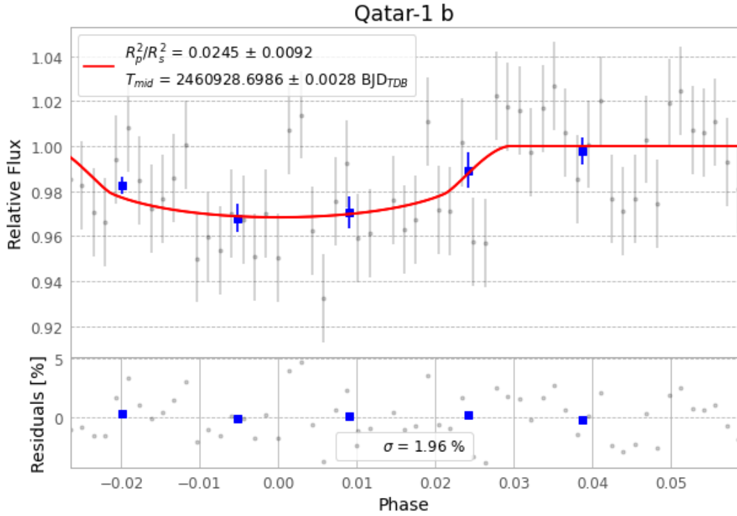
Figure 1 — FinalLightCurve_Qatar-1 b_2025-09-09.png (SHA-256 6dd64be8dc0a6f53...)
