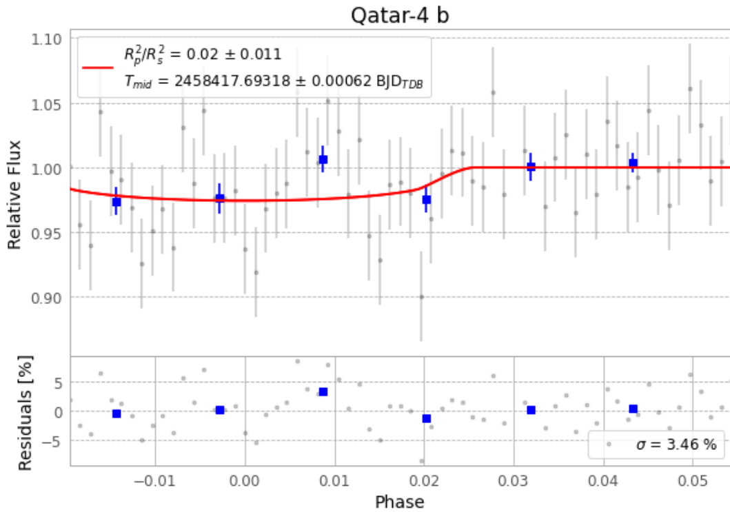
Figure 1 — FinalLightCurve_Qatar-4 b_2018-10-25.png (SHA-256 a196e77e20dad5d6...)
