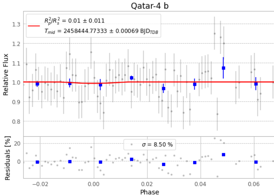
Figure 1 — FinalLightCurve_Qatar-4 b_2018-11-21.png (SHA-256 a6626df418fd19e5...)
