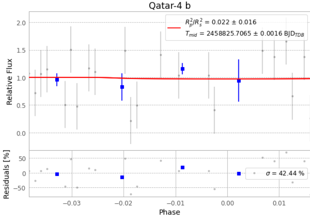
Figure 1 — FinalLightCurve_Qatar-4 b_2019-12-07.png (SHA-256 703a23697b5ccc3b...)
