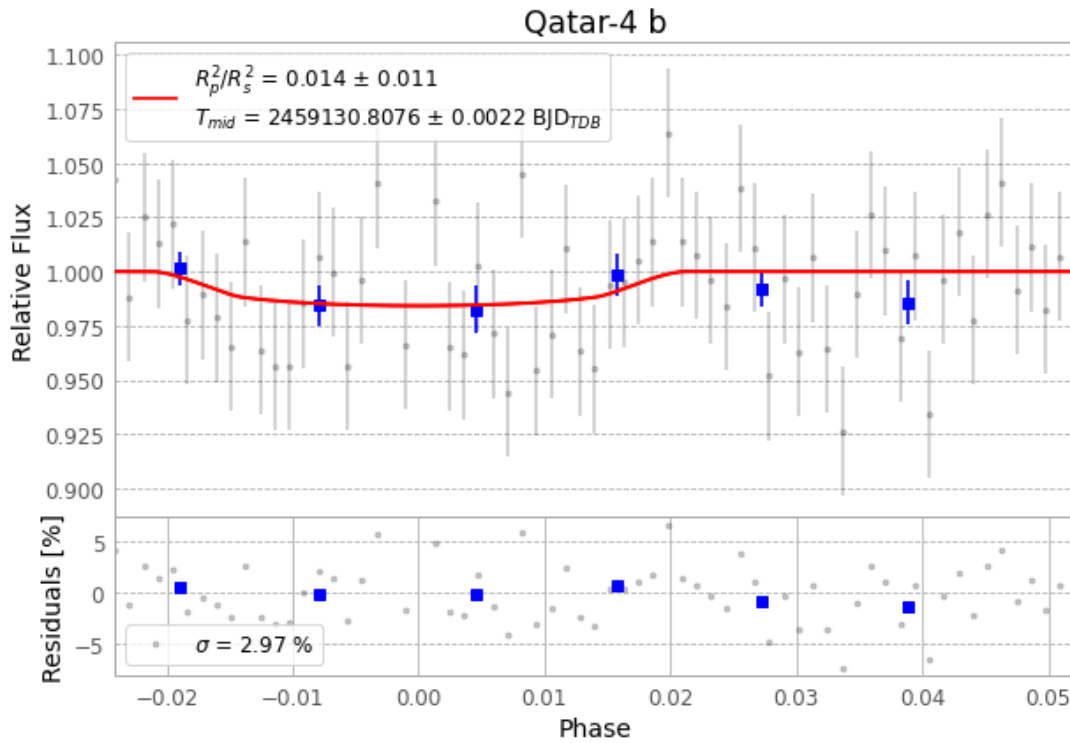
Figure 1 — FinalLightCurve_Qatar-4 b_2020-10-07.png (SHA-256 8df7fd7677ea80b9...)
