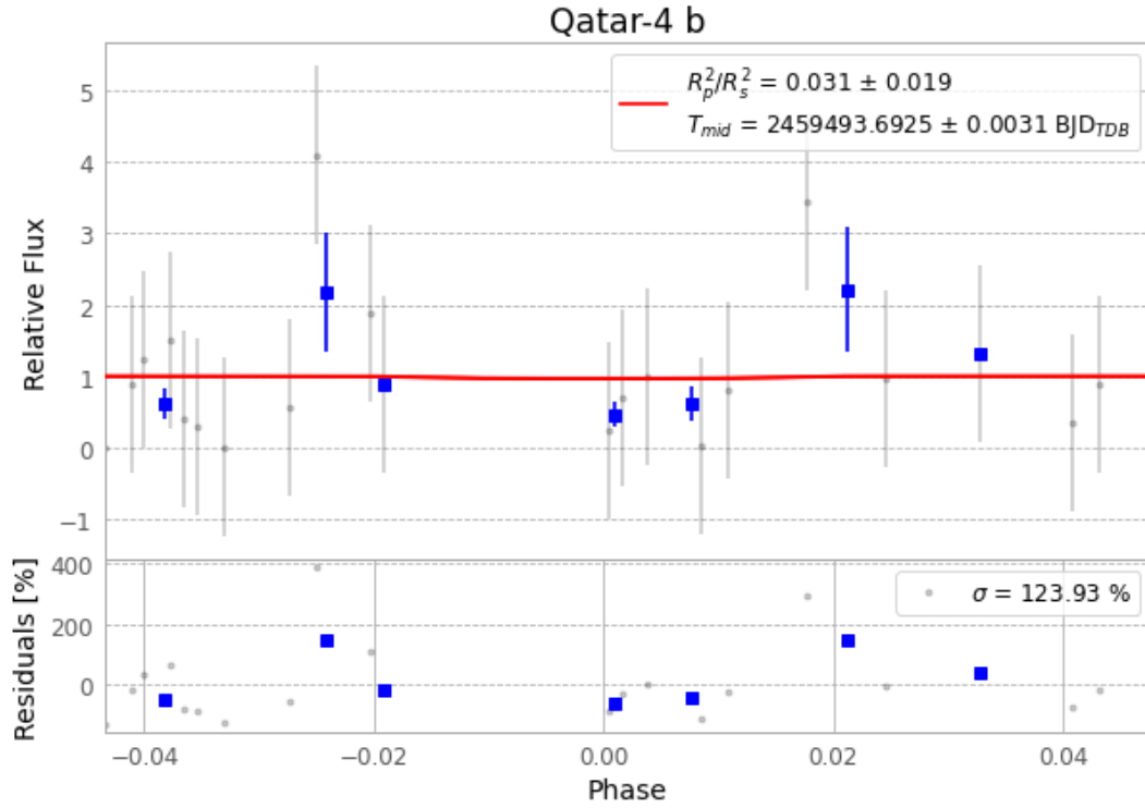
Figure 1 — FinalLightCurve_Qatar-4 b_2021-10-05.png (SHA-256 44c4e131b5ff4376...)
