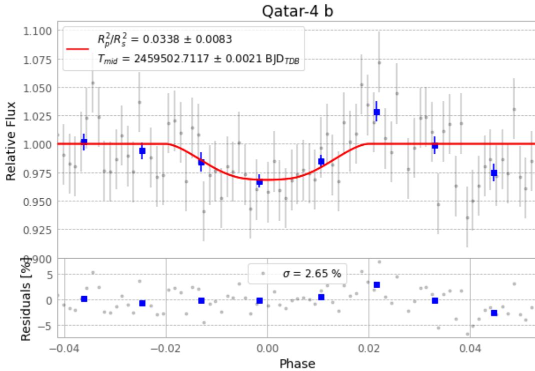
Figure 1 — FinalLightCurve_Qatar-4 b_2021-10-14.png (SHA-256 cb043d05b320cb5c...)
