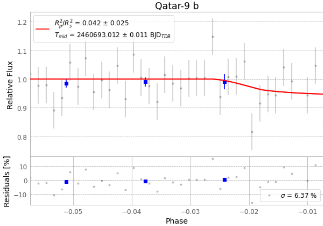
Figure 1 — FinalLightCurve_Qatar-9 b_2025-01-17.png (SHA-256 d43a33fbf6d95a04...)
