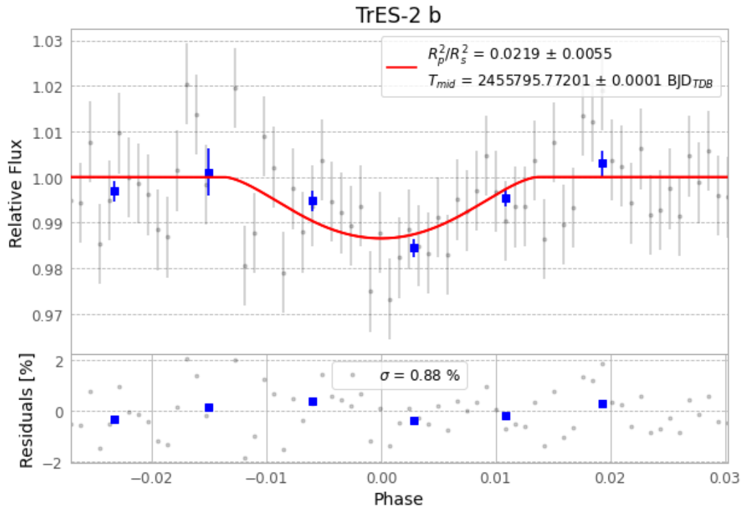
Figure 1 — FinalLightCurve_TrES-2 b_2011-08-21.png (SHA-256 7e4f4d34ab61404a...)
