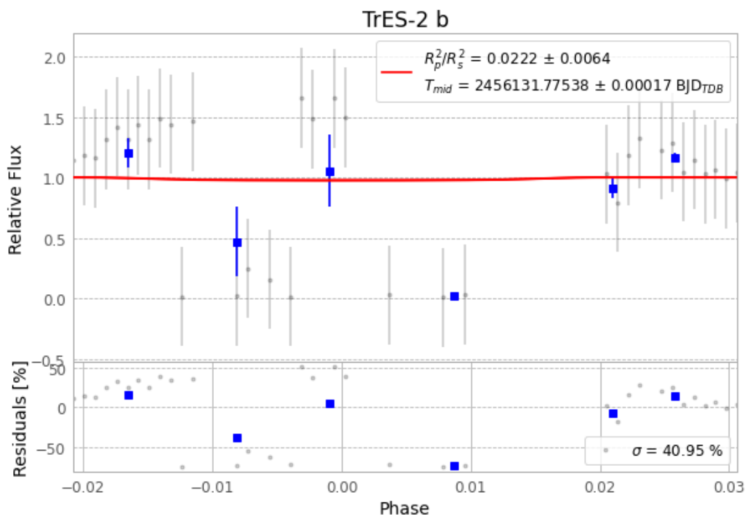
Figure 1 — FinalLightCurve_TrES-2 b_2012-07-22.png (SHA-256 43f2394cbf9ef02b...)
