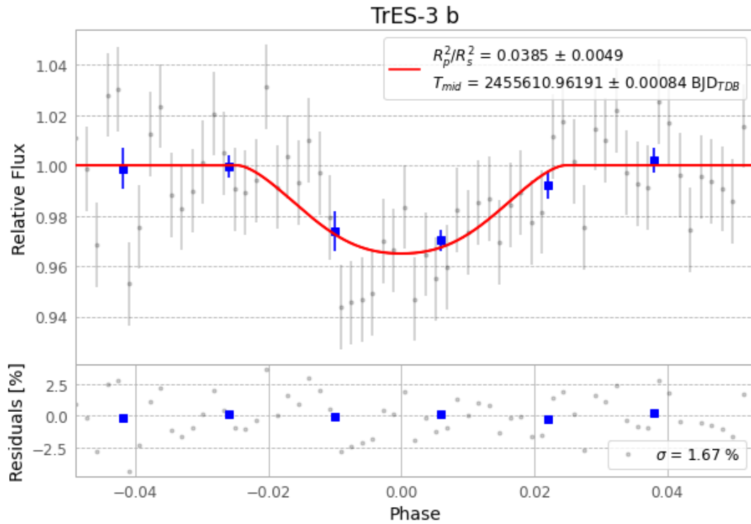
Figure 1 — FinalLightCurve_TrES-3 b_2011-02-18.png (SHA-256 30f3a5fab7fd2bca...)
